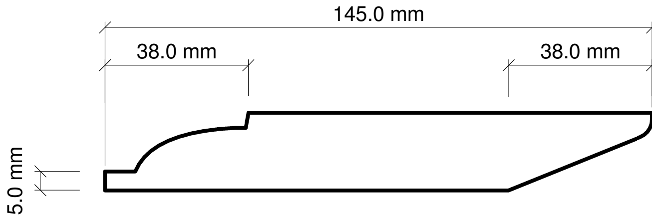
35419 Redwood Ovolo / Chamfered Skirting Premier Grade 20.5mm x 145mm PEFC
