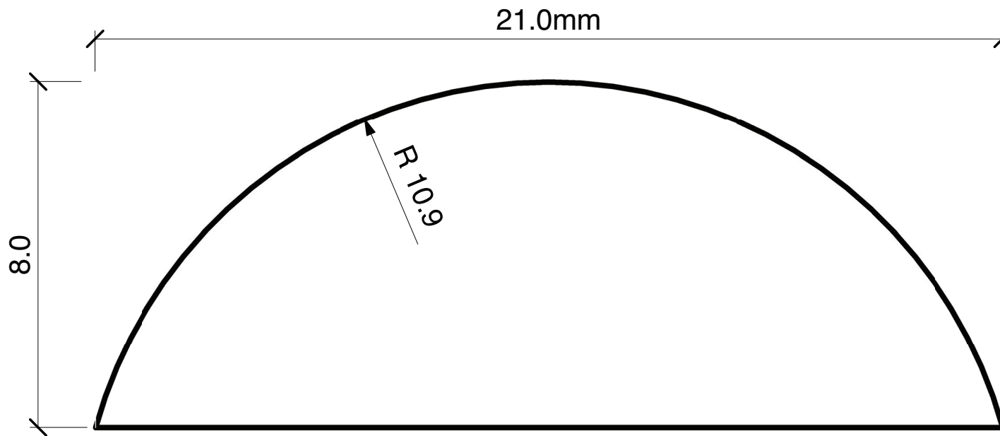
35392 Redwood Half Round Premier Grade 8mm x 21mm PEFC
