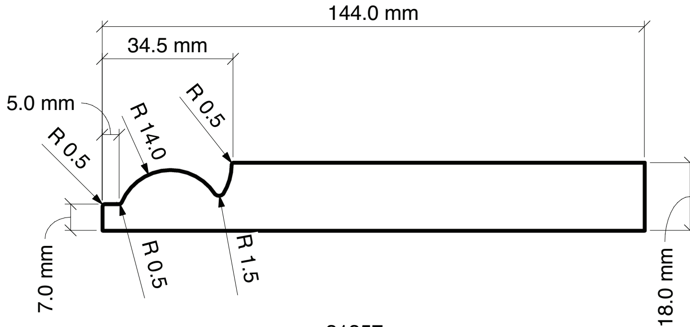
31357 MDF Skirting Torus Primed White 18 mm x 144 mm FSC
