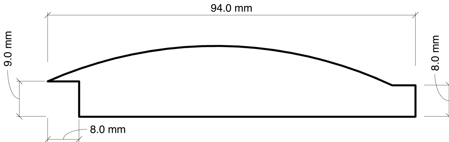
100245 Softwood Pine Shiplap 15 mm x 94 mm
